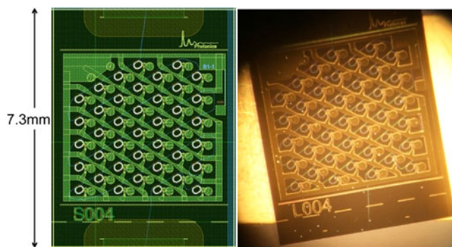
Fig. 2. Layout and photograph of a 40 microresonator TTD device.
