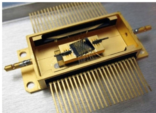
Fig. 3. Photograph showing the inside of a packaged TTD device.
