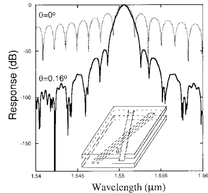
Fig. 4. The response of an X-crossing fused vertical coupler filter with \theta = 0^\circ and 0.16^\circ . d_s = 1.2 \mu\text{m} . The insert is the schematic drawing of X-crossing fused vertical coupler filter.
