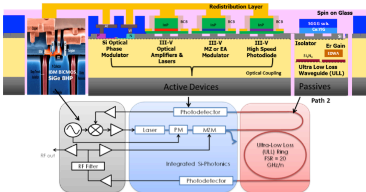
Figure 1: An example of heterogeneous integration to combine low loss \text{Si}_3\text{N}_4 waveguides with Si waveguides with III-V active elements and electronics to make an optoelectronic oscillator.
