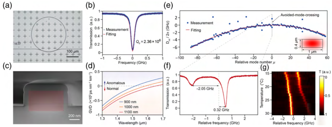
Fig. 1 Resonator characterization. (a) Top-view photograph of the AlGaAsOI microresonator. The radius of the microresonator is 144\ \mu\text{m} , corresponding to 91\ \text{GHz} FSR. Scale bar: 100\ \mu\text{m} . (b) Normalized transmission spectrum of a typical resonance at 1552\ \text{nm} . Lorentzian fitting reveals intrinsic Q factors about 2.36 \times 10^6 . (c) Scanning-electron-microscopy image showing the cross section of the microresonator. The AlGaAs core is highlighted in red, and silica forms the substrate and cladding. Scale bar: 200\ \text{nm} . (d) Calculated dispersion of the TE 0 mode in AlGaAsOI microresonators with respect to the width of the core. The thickness of the core is set as 400\ \text{nm} . The inset shows the corresponding TE 0 mode profile. (e) Measured TE 0 mode family dispersion. D_{\text{int}} = \omega_{\mu} - \omega_0 - D_1\mu = D_2\mu^2/2 + \mathcal{O}(\mu^3) , where \omega_{\mu} is the resonant frequency of the \mu th mode. The index of the mode that is pumped is set to 0, and D_1 is the FSR at pump wavelength. Parabolic fitting (red) shows D_2/2\pi = -1.63\ \text{MHz} . (f) Zoom-in spectrum of the doublet resonances at \mu = 0 indicated in (e). The frequency is plotted relative to the fitting curve. (g) Pseudo-color plot of the relative frequency shifting of the coupled mode pairs from the ideal resonant frequency without the AMX effect, as a function of temperature.
